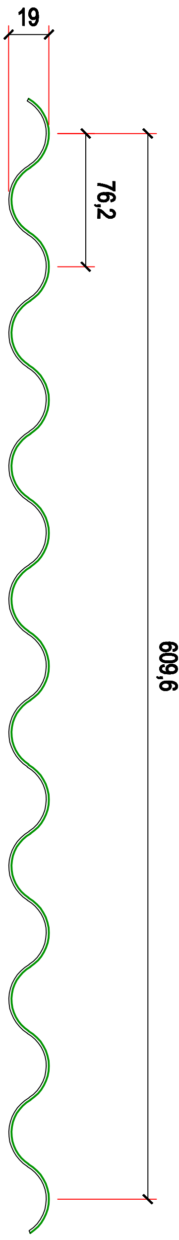
10 / 3 CORRIGATED PROFILE LIPS DOWN
