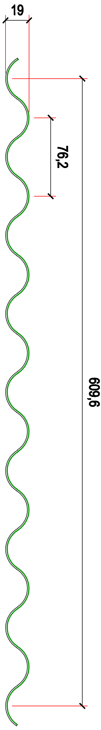
10 / 3 CORRIGATED PROFILE LIPS UP
